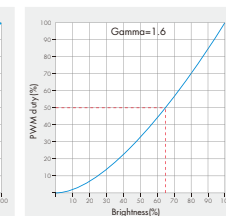
Dimming curve for RGBW/RGB/DM
