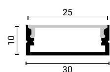
SKU 5116 Black Body- White Cover (L=2m)
