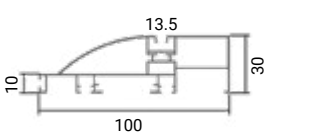
SKU 15123 White Body- White Cover (L=2m)
