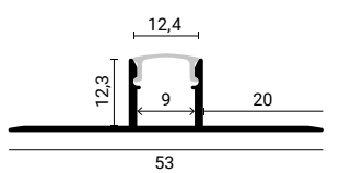
SKU 5112 Silver Body - White Cover (L=2m)
