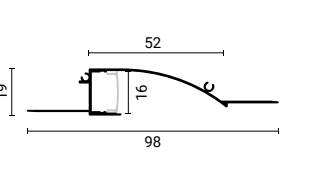
SKU 5128 Silver Body - White Cover (L=2m)
