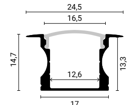
SKU 5108 Silver Body- White Cover (L=2m)
