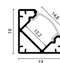
SKU 5100 Black Body- White Cover (L=2m)
