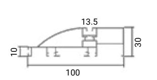
SKU 15122 Black Body- White Cover (L=2m)
