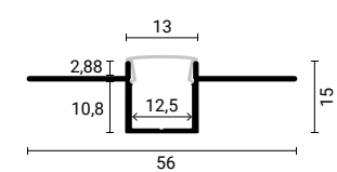
SKU 5162 Silver Body - White Cover (L=2m)
