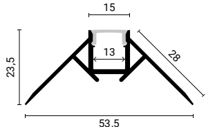
SKU 5165 Silver Body - White Cover (L=2m)
