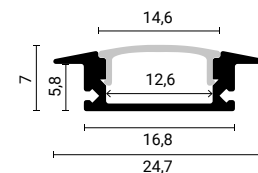
SKU 5106 White Body - White Cover (L=2m)
