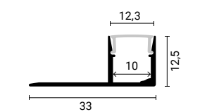
SKU 5111 Silver Body - White Cover (L=2m)
