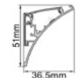
SKU 15135 Silver Body - White Cover (L=2m)
