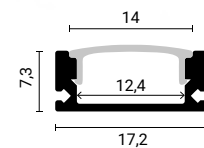
SKU 5190 Silver Body- White Cover (L=1m)
