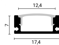
SKU 5185 Black Body- White Cover (L=2m)
