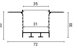
SKU 5124 Black Body - Black Cover (L=2m)
