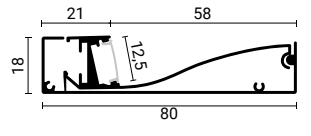
SKU 15115 Silver Body- White Cover (L=2m)
