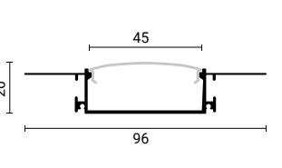
SKU 5134 Silver Body - White Cover (L=2m)
