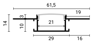
SKU 5145 Silver Body - White Cover (L=2m)
