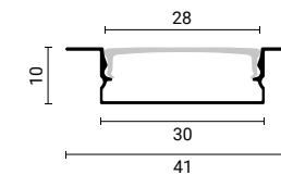
SKU 5119 Black Body- White Cover (L=2m)
