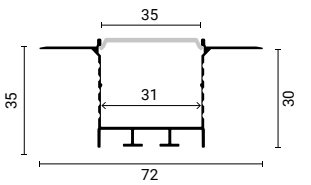
SKU 5123 Silver Body - White Cover (L=2m)
