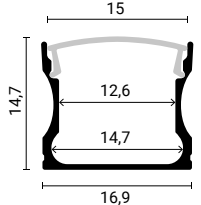
SKU 5175 Silver Body- White Cover (L=2m)
