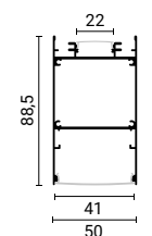
SKU 15129 Marble Body- White Cover (L=2m)
