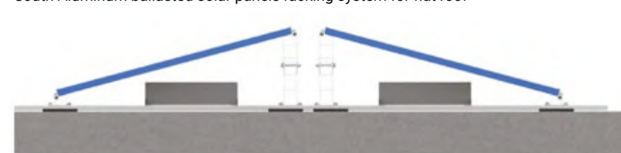
South Aluminum ballasted solar panels racking system for flat roof
