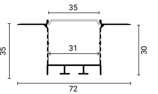
SKU 5125 Black Body - White Cover (L=2m)
