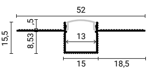
SKU 15112 Silver Body - Black Cover (L=2m)
