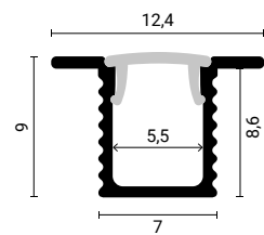
SKU 5141 Silver Body- White Cover (L=2m)
