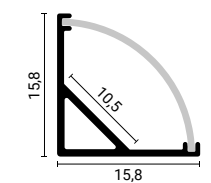
SKU 5150 Silver Body- White Cover (L=2m)
