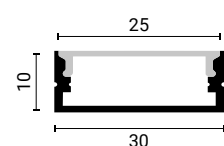
SKU 5114 Black Body- Black Cover (L=2m)
