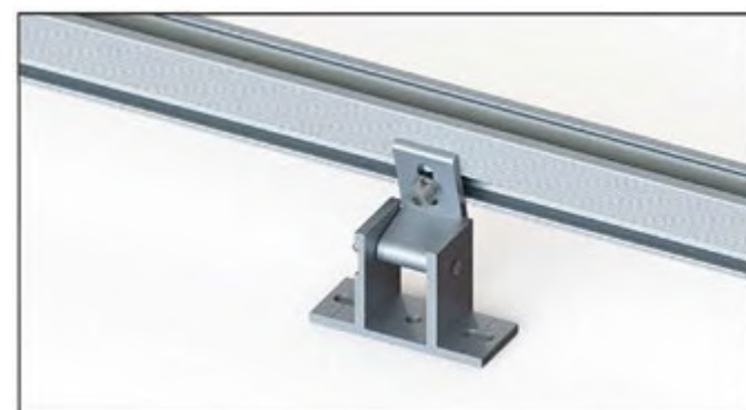
Step 1: Fix adjustable front leg and rear leg on steel roofing.
