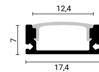
SKU 5107 Black Body- Black Cover (L=2m)
