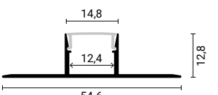
SKU 5143 Silver Body - White Cover (L=2m)
