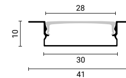
SKU 5118 Silver Body- White Cover (L=2m)
