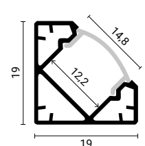
SKU 5101 Black Body - Black Cover (L=2m)
