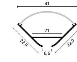
SKU 5110 Silver Body- White Cover (L=2m)
