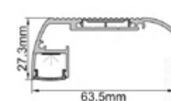
SKU 15134 Black Body - White Cover (L=2m)
