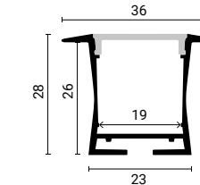
SKU 5130 Silver Body- White Cover (L=2m)
