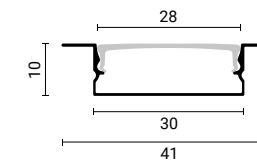
SKU 5117 Black Body- Black Cover (L=2m)
