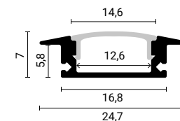
SKU 5105 Black Body - Black Cover (L=2m)
