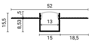
SKU 15111 Silver Body - White Cover (L=2m)
