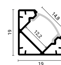
SKU 5102 White Body- White Cover (L=2m)
