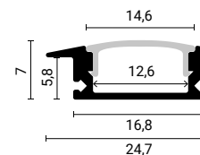
SKU 5104 Black Body - White Cover (L=2m)
