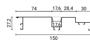
SKU 15113 White Body- White Cover (L=2m)
