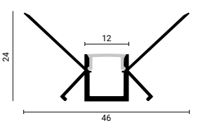
SKU 5166 Black Body - White Cover (L=2m)
