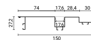
SKU 15114 White Body- Black Cover (L=2m)
