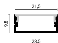
SKU 5183 Black Body- Black Cover (L=2m)
