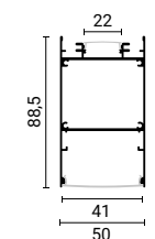
SKU 15128 White Body- White Cover (L=2m)
