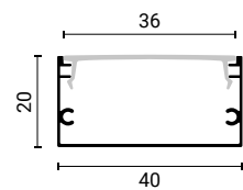
SKU 5121 Silver Body- White Cover (L=2m)
