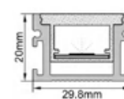
SKU 15133 Silver Body - White Cover (L=2m)
