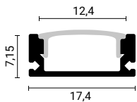
SKU 5184 White Body- White Cover (L=2m)
