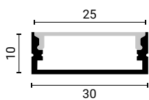
SKU 5116 Black Body- White Cover (L=2m)
