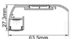
SKU 15134 Black Body - White Cover (L=2m)
