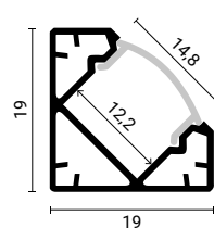
SKU 5101 Black Body - Black Cover (L=2m)
