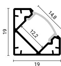
SKU 5102 White Body- White Cover (L=2m)
