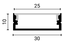
SKU 5115 Silver Body- White Cover (L=2m)
