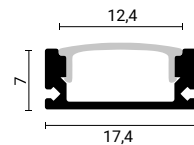
SKU 5107 Black Body- Black Cover (L=2m)
