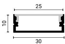
SKU 5114 Black Body- Black Cover (L=2m)
