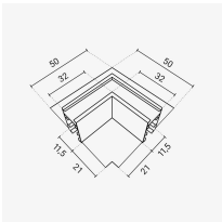
Angle horizontal M05-R
